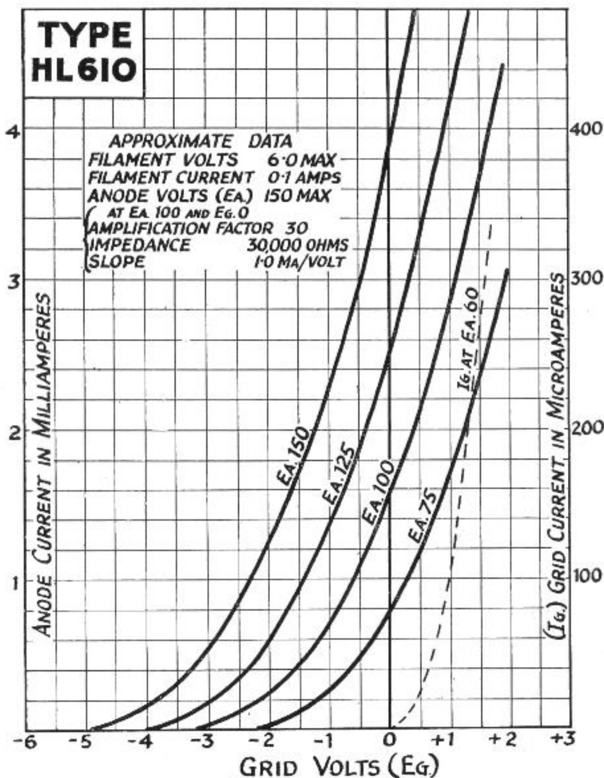
Characteristic Curve of Average HL 610 Valve.
